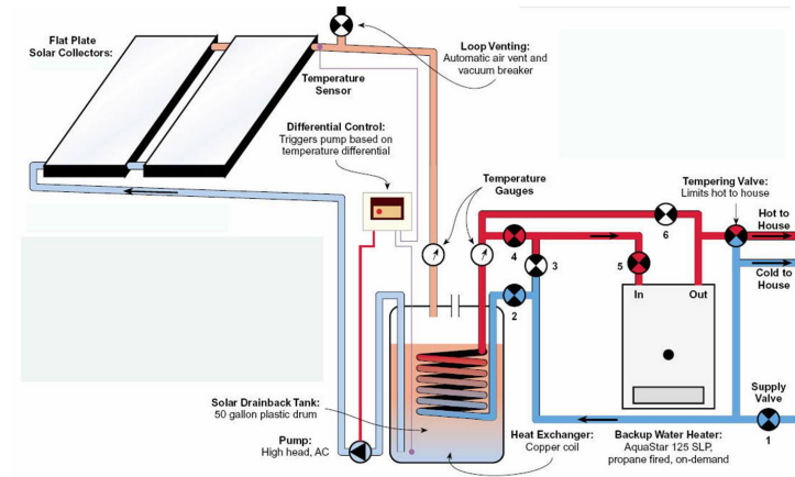
SOLAR DOMESTIC HOT WATER SYSTEM
