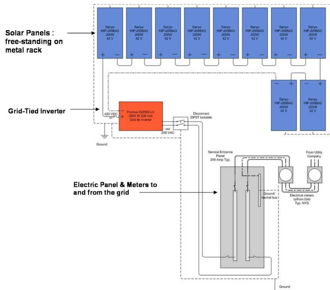
FUTURE SOLAR PHOTOVOLTAIC — GRID TIED SYSTEM
